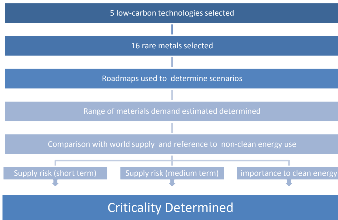
Figure 54: Criticality assessment methodology employed by Critical Materials Strategy, USA, 2011
