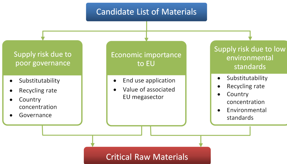
Figure 51: Schematic of EU criticality methodology
