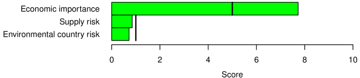
Figure 43: Results of the criticality assessment for natural rubber
